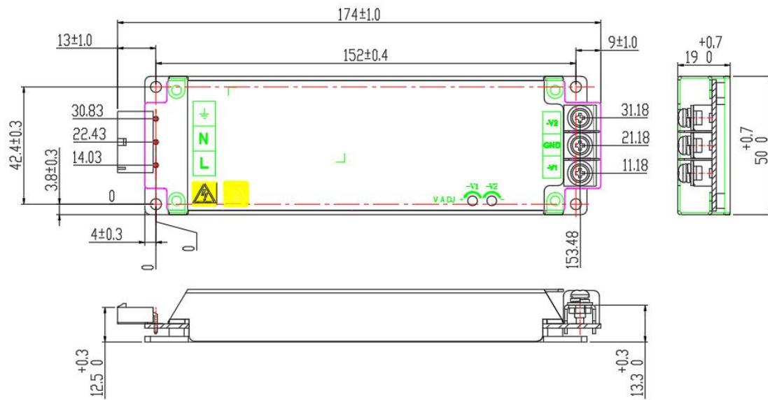
Definition and Installation Notes for Input Terminal and Output Terminal
